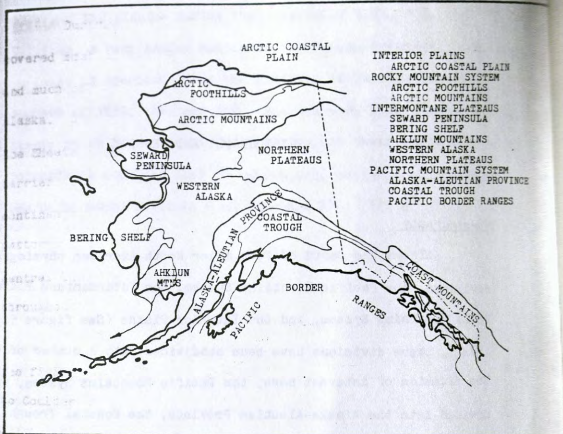
Figure 5. The Physiographic Provinces of Alaska (Wahrhaftig 1965).
