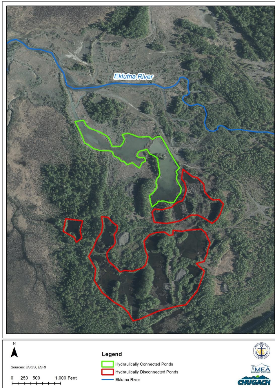
Figure 3-4 Off Channel Ponds located in Reach 3 of the Eklutna River. Some of these ponds may become physically connected to the river via surface flows, while others may remain disconnected with water levels influenced by groundwater from other sources or hyporheic underflow from the river.
