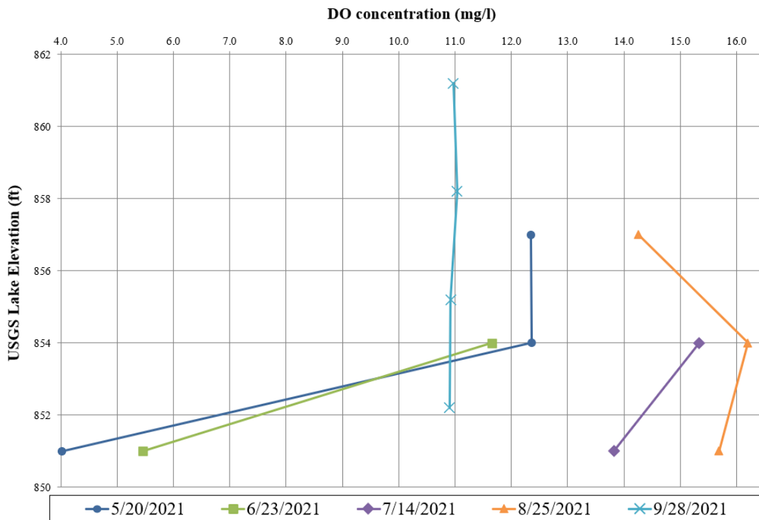
Figure 5-11. Eklutna Pond – monthly dissolved oxygen concentration profiles, 2021.
