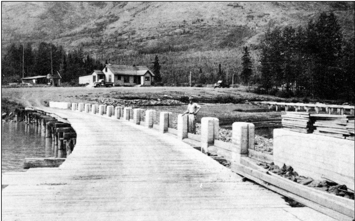
Figure 5.2-16. View of Storage Dam (Feature 2, center); “breakwater weir” (Feature 1, right); and caretaker’s house. From USBR (1948).
