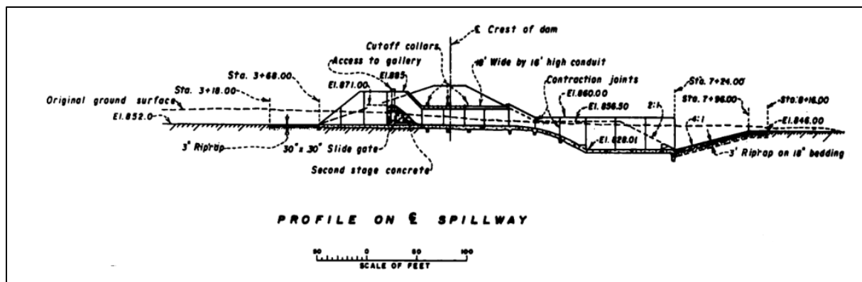
Figure 2.2-6. Profile view of new dam and spillway construction (USBR 1967:Figure 22).
